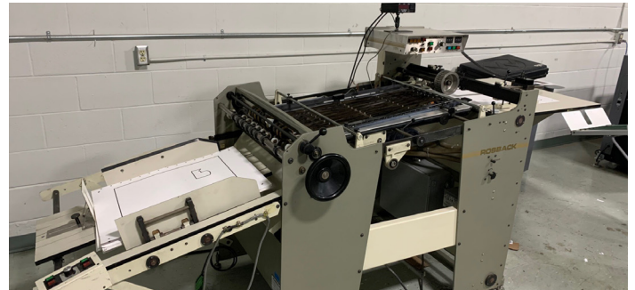
Rosback 240B Vacuum Feed Slit/Score/Perforation Machine $14,995 $9,995 Slit, score & perf substrates up to 14pt card; sizes from 7.5" x 7.5" up to 30" x 30"; up to 25k ft/hr
